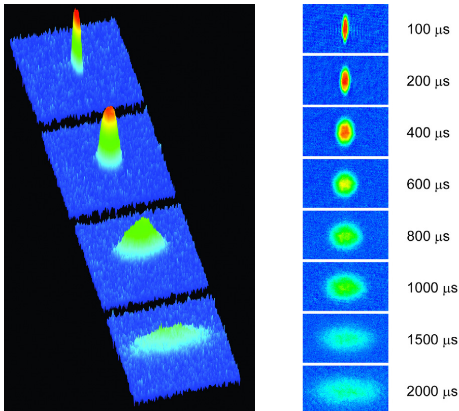
Figure 4. Experimental images. Elliptic flow of a strongly interacting Fermi gas as a function of time after release from a cigar-shaped optical trap: from top to bottom, 100 \mu\text{s} to 2 \text{ ms} after release. The pressure gradient is much larger in the initially narrow directions of the cloud than in the long direction, causing the gas to expand much more rapidly along the initially narrow directions, inverting the aspect ratio. Achieving a nearly perfect elliptic flow requires extremely low shear viscosity, as is the case for a QGP. The sequence of images is created by recreating similar initial conditions and destructively imaging the cloud at different times after release [46].
